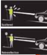
Scattered vs Retroreflection
